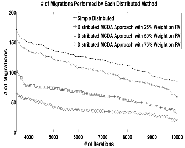
Fig. 8. A view of our approach using different weight assignments to resource variation criteria and SDM in terms of the number of migrations.
